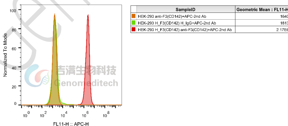
Figure 2 | H_F3(CD142) HEK-293 Cell Line (Cat. GM-C39989) was determined by flow cytometry using Anti-H_F3(CD142) hIgG1 Antibody(Tisotumab) (Cat. GM-28928AB ).
