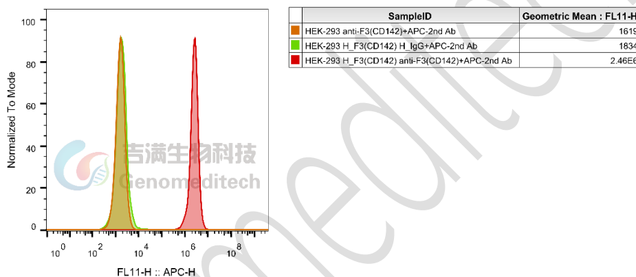
Figure 1 | H_F3(CD142) HEK-293 Cell Line (Cat. GM-C39989) was determined by flow cytometry using Anti-F3(CD142) hIgG1 Reference Antibody (Tisbio) (Cat. GM-87834MAB ).
